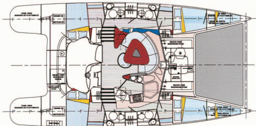
BAHIA 46
